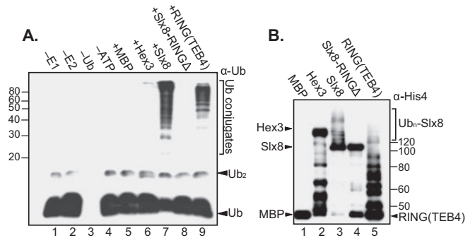
FIGURE 5. Slx8, but not Hex3, exhibits self-ubiquitination activity in vitro . A , purified recombinant Hex3, Slx8, Slx8-RING \Delta , MBP, and RING(TEB4) were used in an in vitro auto-ubiquitination (Ub) assay. Lane 5–9, the recombinant proteins listed were mixed in a reaction buffer containing E1 (Uba1), E2 (Ubc4), ubiquitin, and ATP. Control reactions are depicted in lanes 1–4. Samples from individual reactions were resolved by 16.5% Tricine SDS-PAGE and immunoblotted with anti-ubiquitin antibodies ( \alpha -Ub). The purified RING domain of TEB4 was included as a positive control (lane 9). Mono-, di-, and higher order ubiquitin conjugates are indicated. B , samples from A were resolved on an 8% SDS-PAGE gel and immunoblotted with an anti-His4 antibody to detect the purified His 6 -tagged proteins shown.
