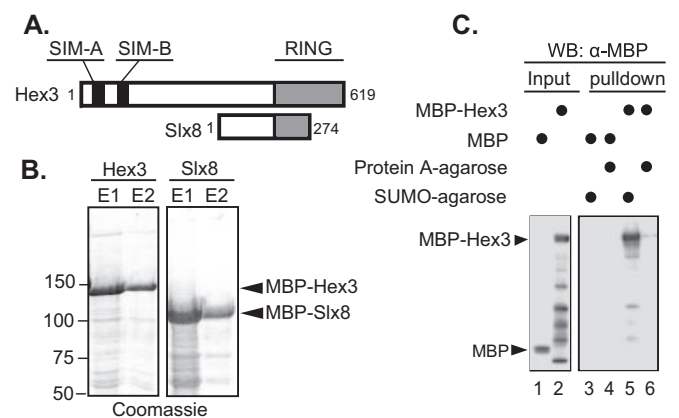
FIGURE 2. Recombinant Hex3 interacts with SUMO in vitro . A , schematic of Hex3 and Slx8 proteins with Hex3 SIMs and RING domains highlighted. B , purification of MBP fusions of Hex3 and Slx8 from E. coli cell extracts. Proteins were harvested from multiple elutions with maltose-containing buffer. Elutions 1 and 2 ( E1 , E2 ) were resolved by 8% SDS-PAGE. Size standards are indicated on the left. C , direct interaction between Hex3 and SUMO was determined by an in vitro pull-down assay. Recombinant MBP (New England Biolabs) and MBP-Hex3 were incubated with either SUMO-1-agarose or protein A-agarose. Precipitated proteins were run on 8% SDS-PAGE gels and detected by anti-MBP (Santa Cruz) immunoblotting (WB, lanes 3–6). Lanes 1–2, input (3.33%) MBP and MBP-Hex3.
