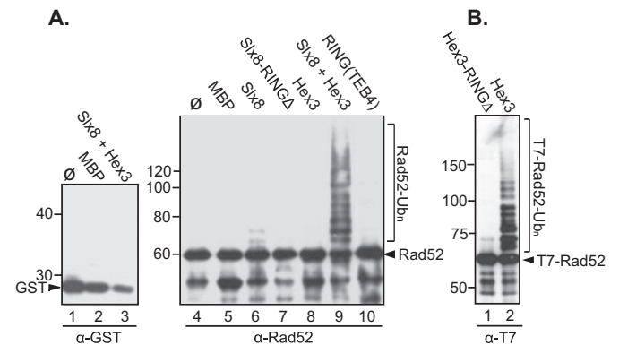
FIGURE 6. Yeast Rad52 protein is a substrate for Hex3-Slx8-mediated ubiquitination. A , recombinant yeast Rad52 (0.2 \mu M) was incubated at 30 °C for 2 h with E1 (Uba1), E2 (Ubc4), and 0.4 \mu M of the indicated recombinant proteins (lane 5–10). Control reactions lacking E3 or with MBP (lanes 4–5) or containing purified GST in place of Rad52 (lane 1–3) are also shown. B , equal amounts (0.4 \mu M) of recombinant Hex3 or Hex3-RING \Delta were supplied to separate ubiquitination reactions containing Uba1, Ubc4, Slx8, and 0.2 \mu M T7-tagged recombinant Rad52. Reaction products were examined by anti-T7 immunoblotting. GST, glutathione S-transferase.
